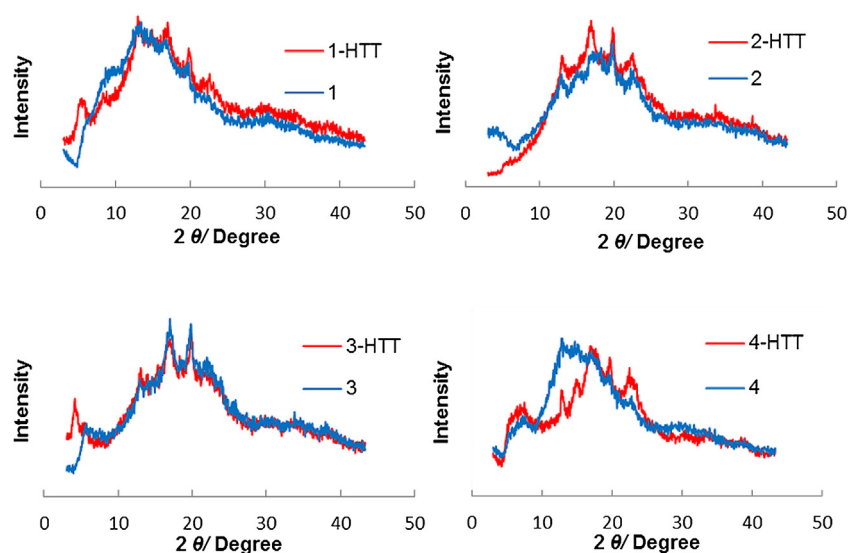
Fig. 4. X-ray diffractograms of compression molded normal maize starch extrudate before and after hydrothermal treatment (HTT). The extrusion processing conditions of films prior to compression molding are listed in Table 3.
