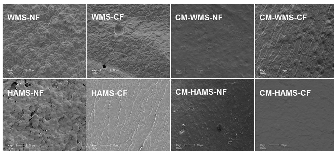
Fig. 1. SEM images of non-fractured (NF) and cryo-fractured (CF) surfaces of waxy and high-amylose maize starch (WMS and HAMS, respectively) films before and after compression molding (CM).
