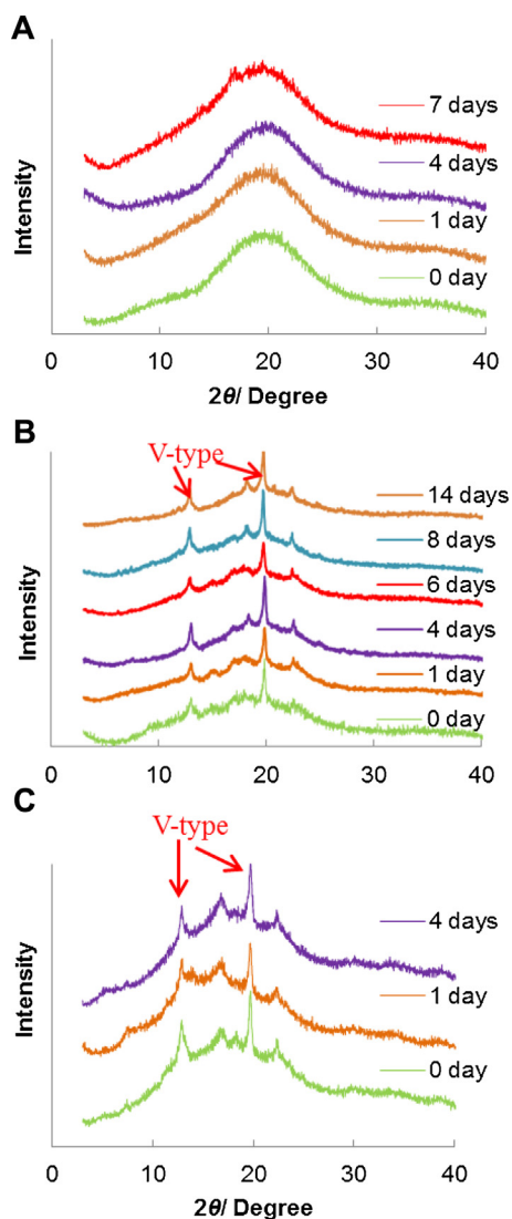
Fig. 3. X-ray diffractograms of compression molded starch films after being stored for different times at 54% RH. Red arrows point at the peaks of V-type crystallinity. (A for waxy maize starch films, B for normal maize starch films, and C for high-amylose maize starch films).
